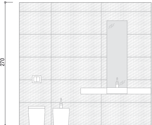
Wall C
