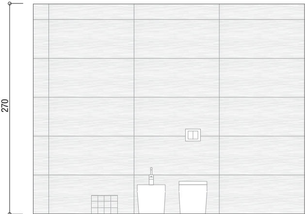
Wall A
