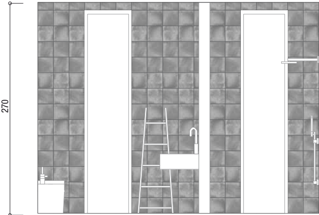
Wall B
