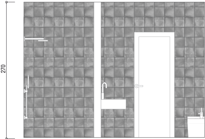
Wall D
